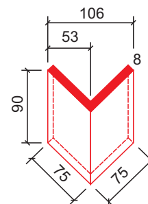
DETALLE ANGULAR
